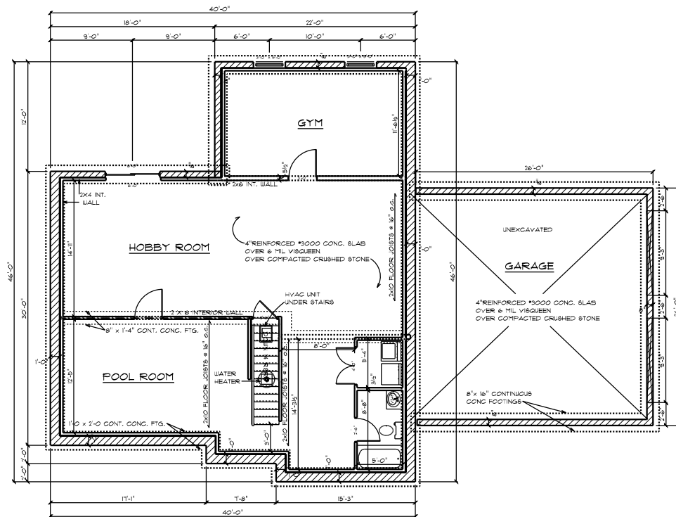
FOUNDATION PLAN
