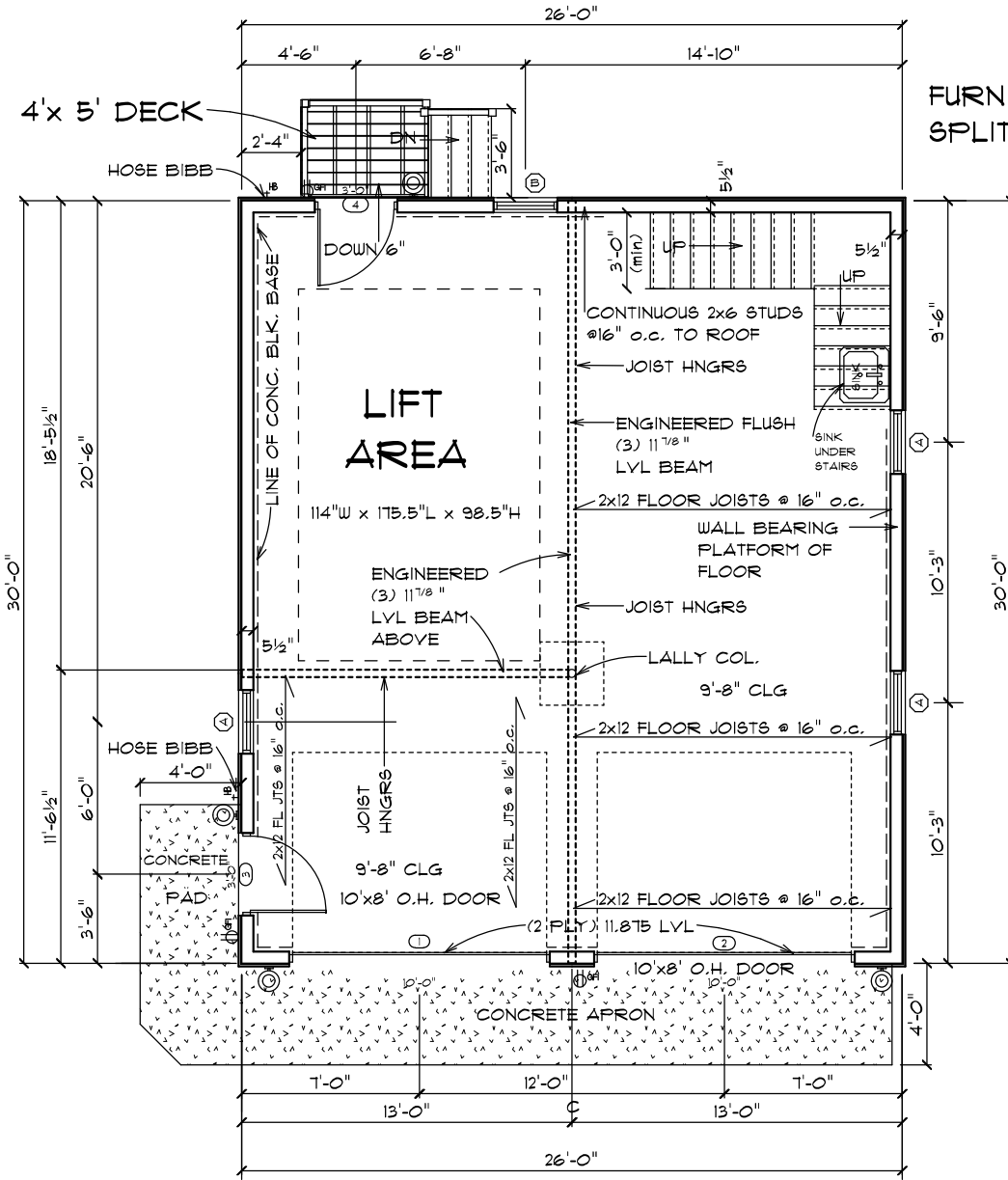
FLOOR PLAN
